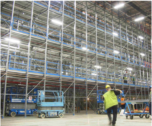
Multi tier installation 4 levels hanging garment storage.
